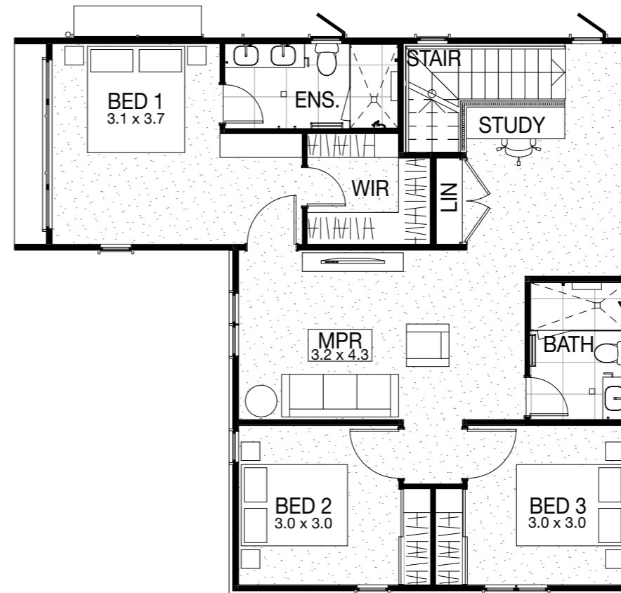
LEVEL 1
