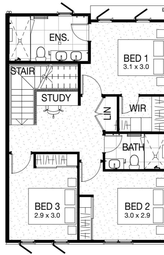
LEVEL 1
