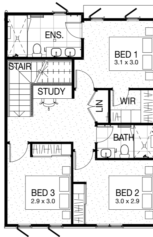
LEVEL 1
