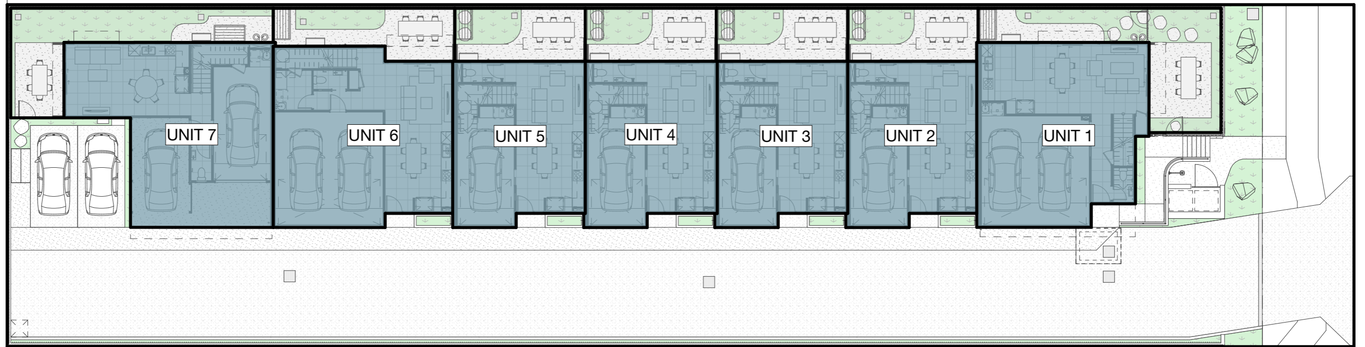
SITE PLAN
